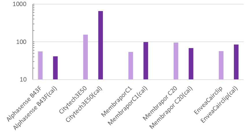
between-sensor uncertainty (%)
